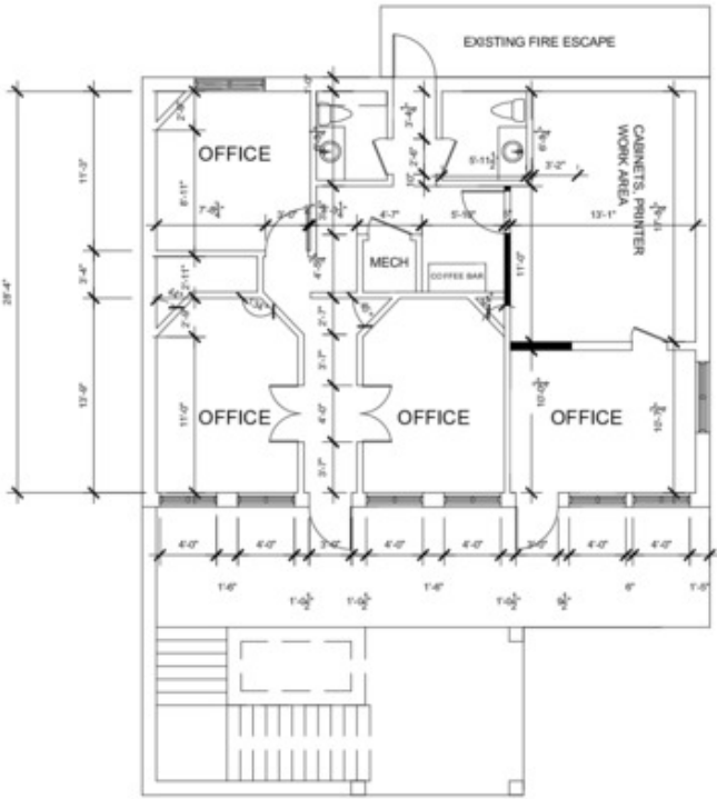
02 EXISTING SECOND FLOOR - FLOOR PLAN SCALE: 1/8" = 1'-0"
