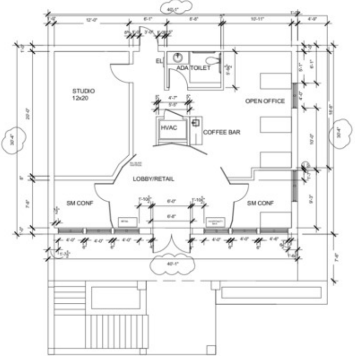
01 EXISTING FIRST FLOOR - FLOOR PLAN SCALE: 1/8" = 1'-0"
