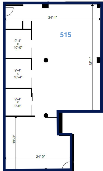
Floor Plan
