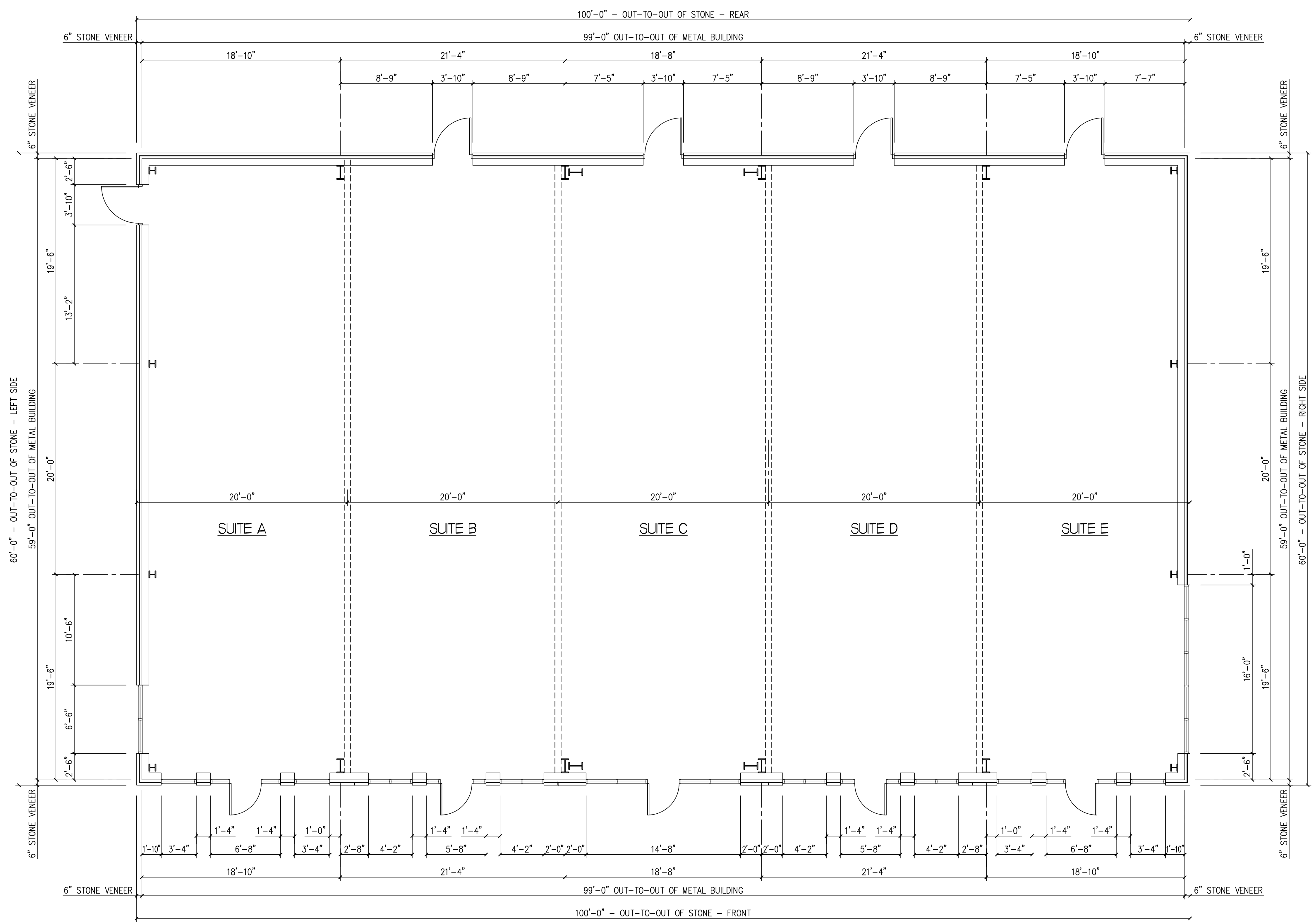
PRELIMINARY FLOOR PLAN SCALE: 3/16" = 1'-0"
