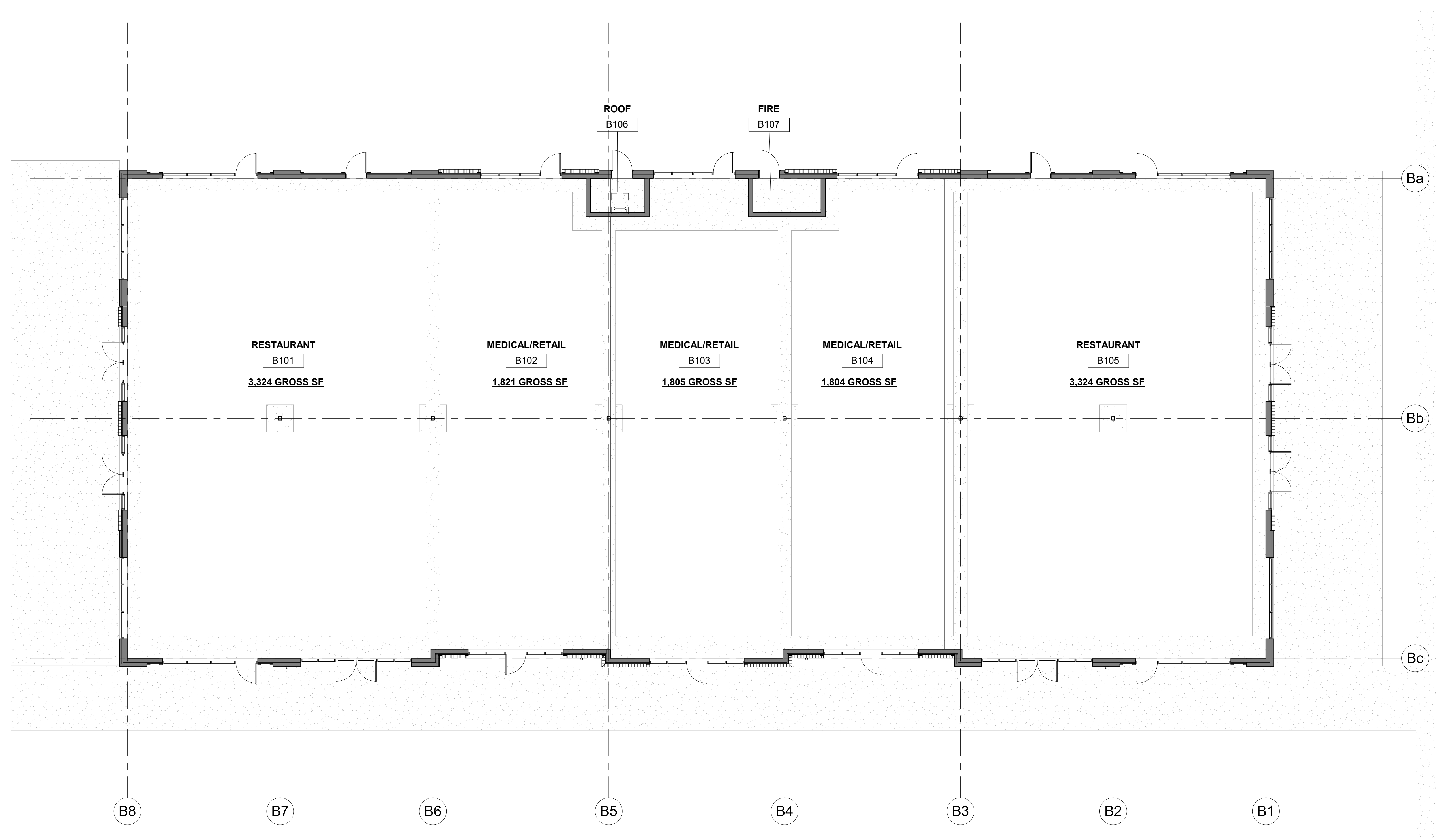
1 BLDG B - GSF EXHIBIT - 10.02.25 1/8" = 1'-0"
