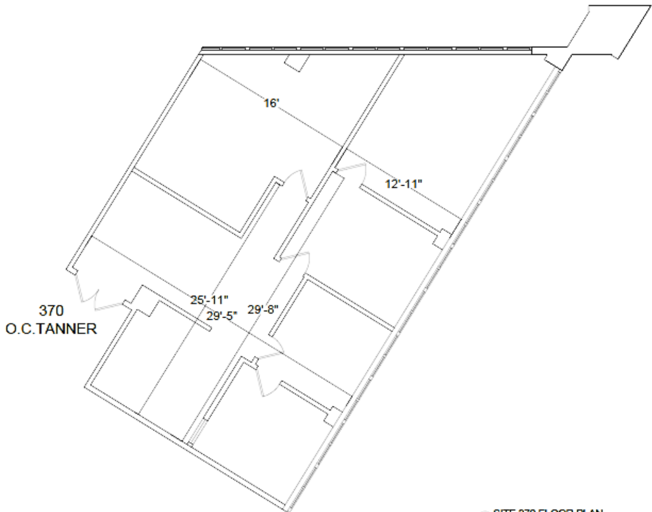
3 SITE 370 FLOOR PLAN 3/16" = 1'-0"
