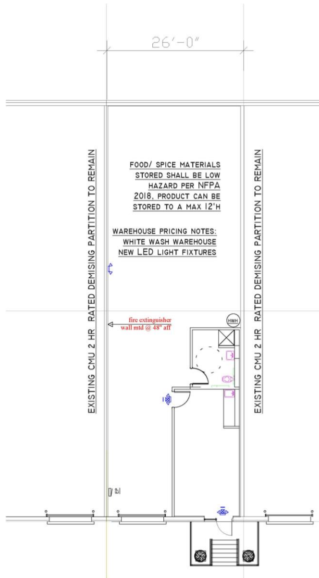
A.3 Overall Office/ Warehouse Plan scale 1 / 8"=1'-0"
