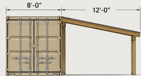
END VIEW (LOOKING FROM REAR)
