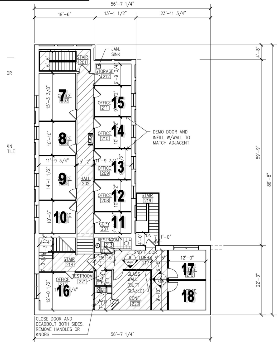
2 SECOND FLOOR PLAN - 3300 SF 1/8" = 1'-0"
