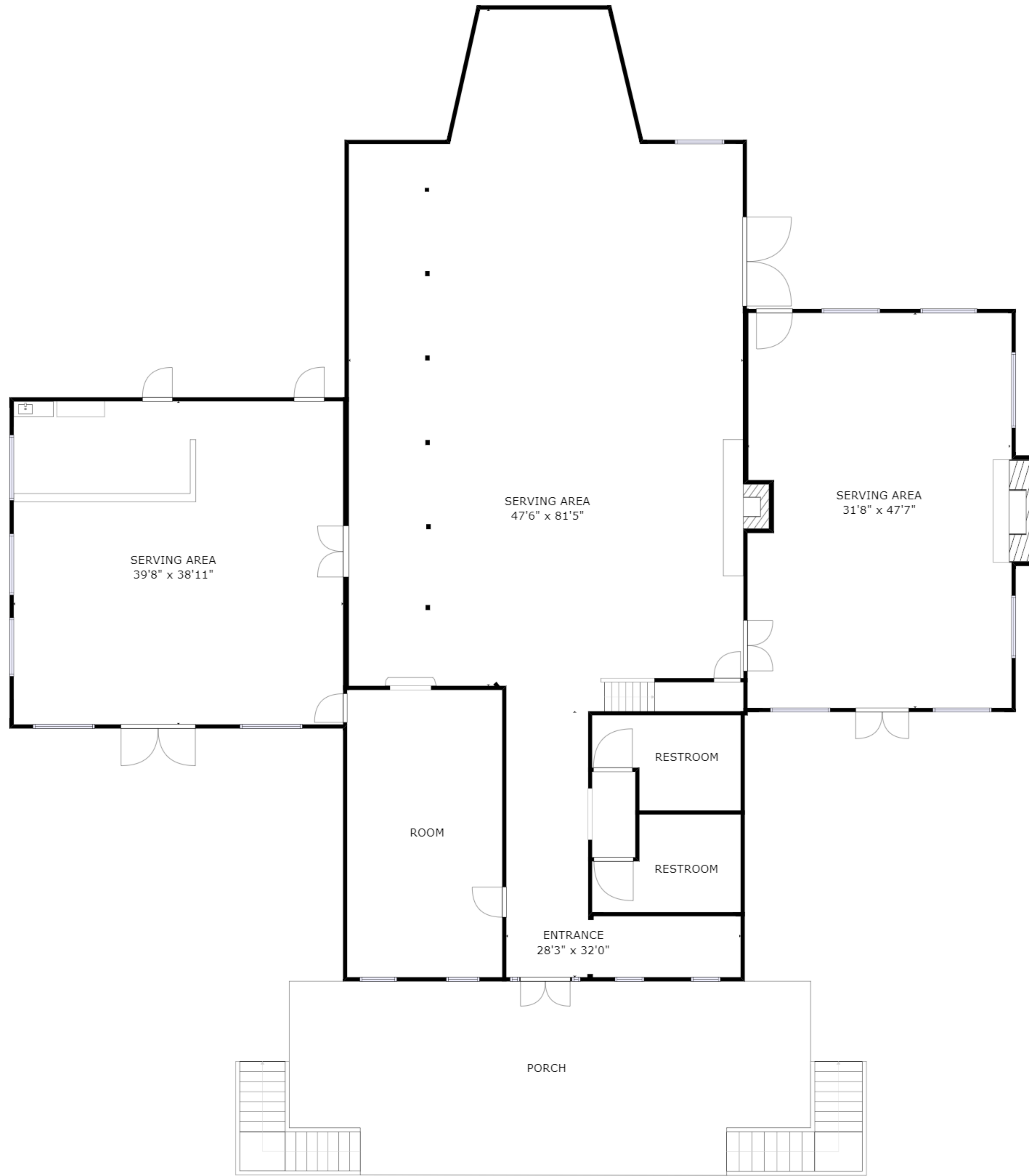
FLOOR 1
