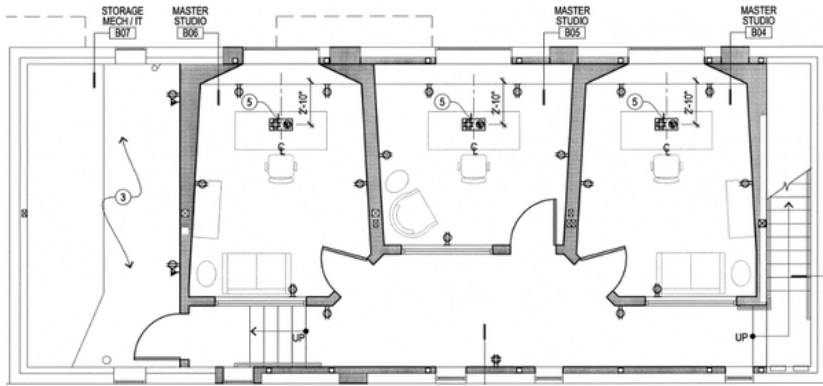
Basement Floorplan
