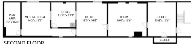
SECOND FLOOR
