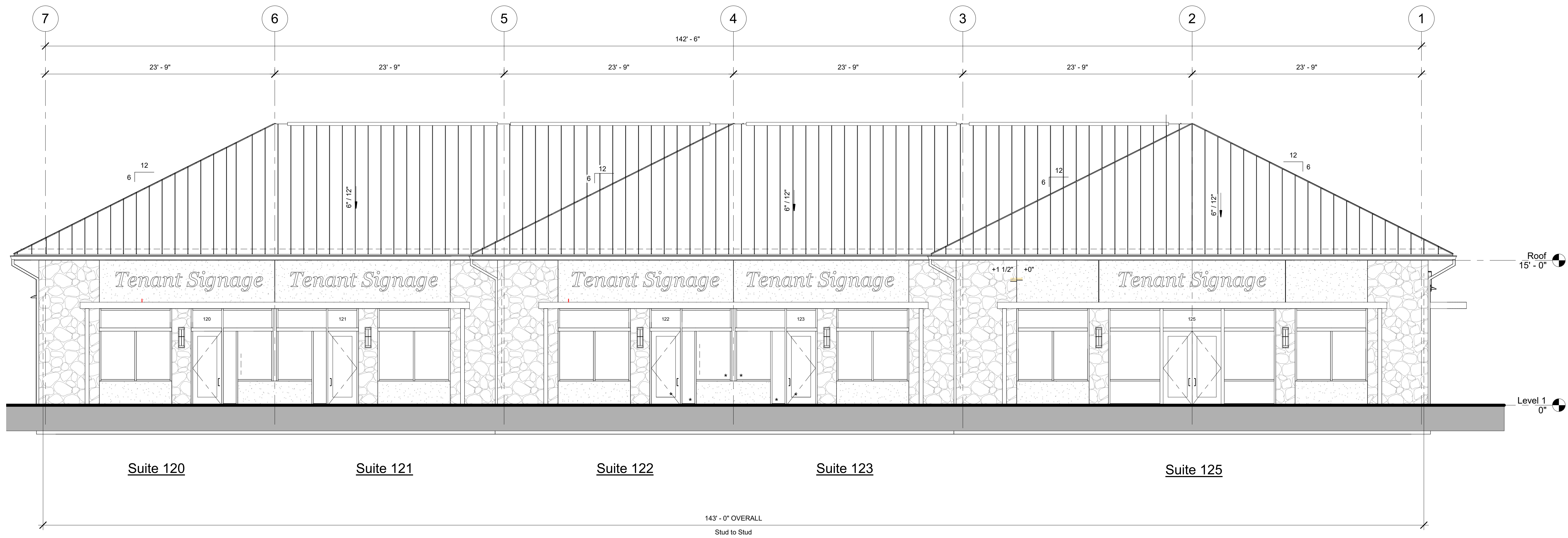
1 Building 3 Lease Front Elevation 3/16" = 1'-0"
