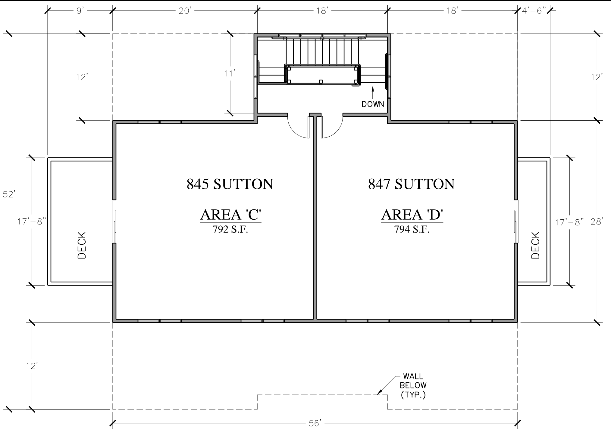
845 & 847 SUTTON - UPSTAIRS FLOOR PLAN
