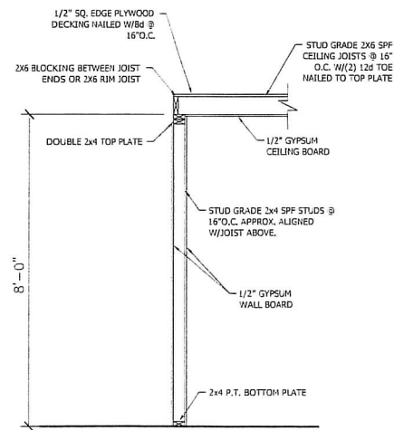
INTERIOR RESTROOM WALL DETAIL SCALE: 1/2" = 1'-0"
