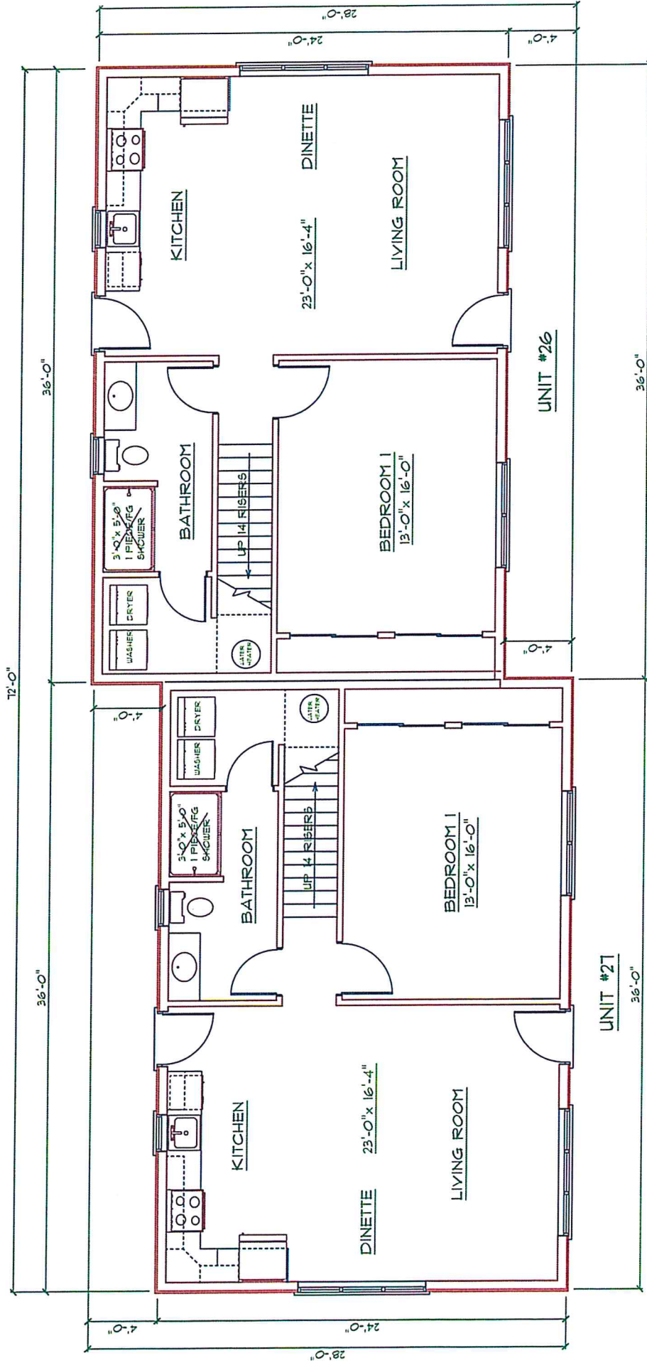
BUILDING C UNIT #26 & UNIT #21 FIRST FLOOR PLAN REVISED 6-01-2023
