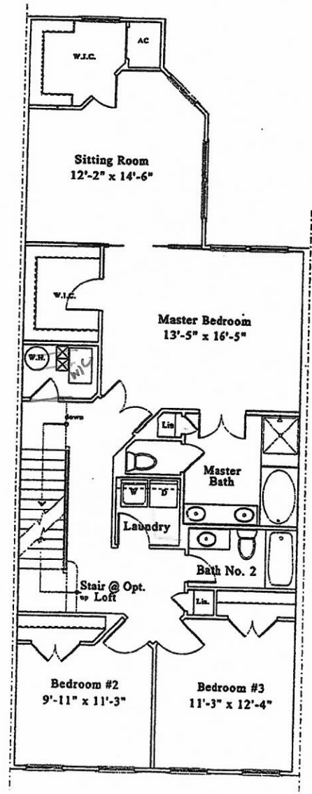
Third Floor 1248 sq. ft.
