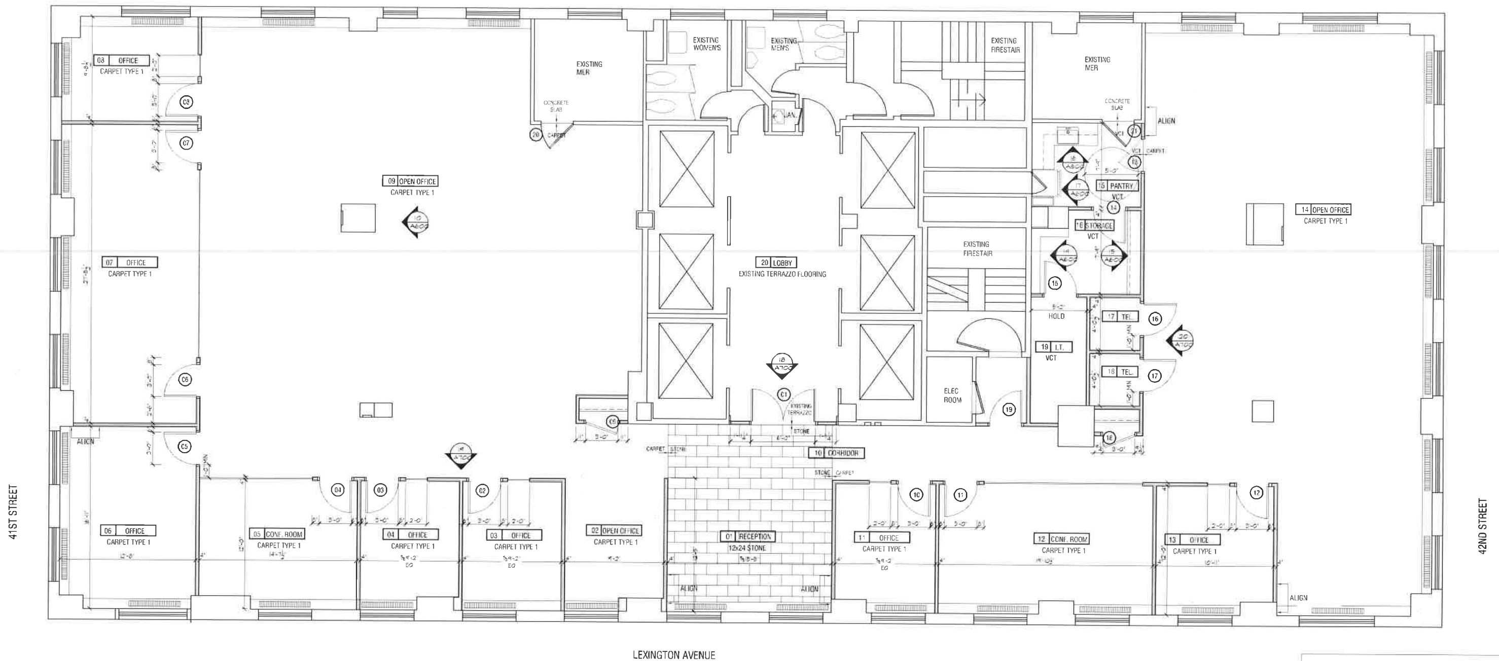
1 34TH FLOOR CONSTRUCTION PLAN SCALE: 1/4" = 1'-0"
