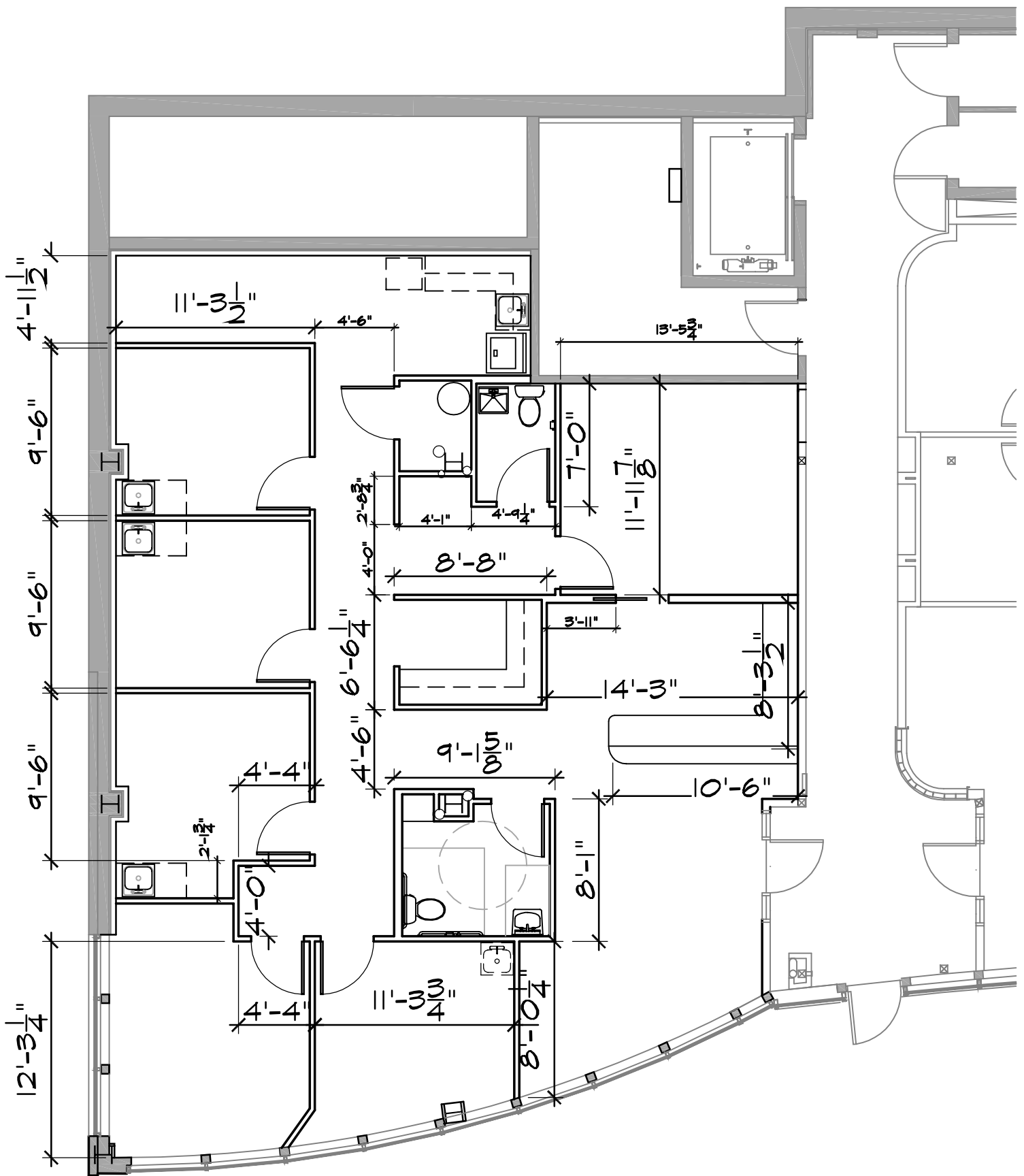
LOWER LEVEL SOUTH FLOOR PLAN 1,920 SQ. FT.
