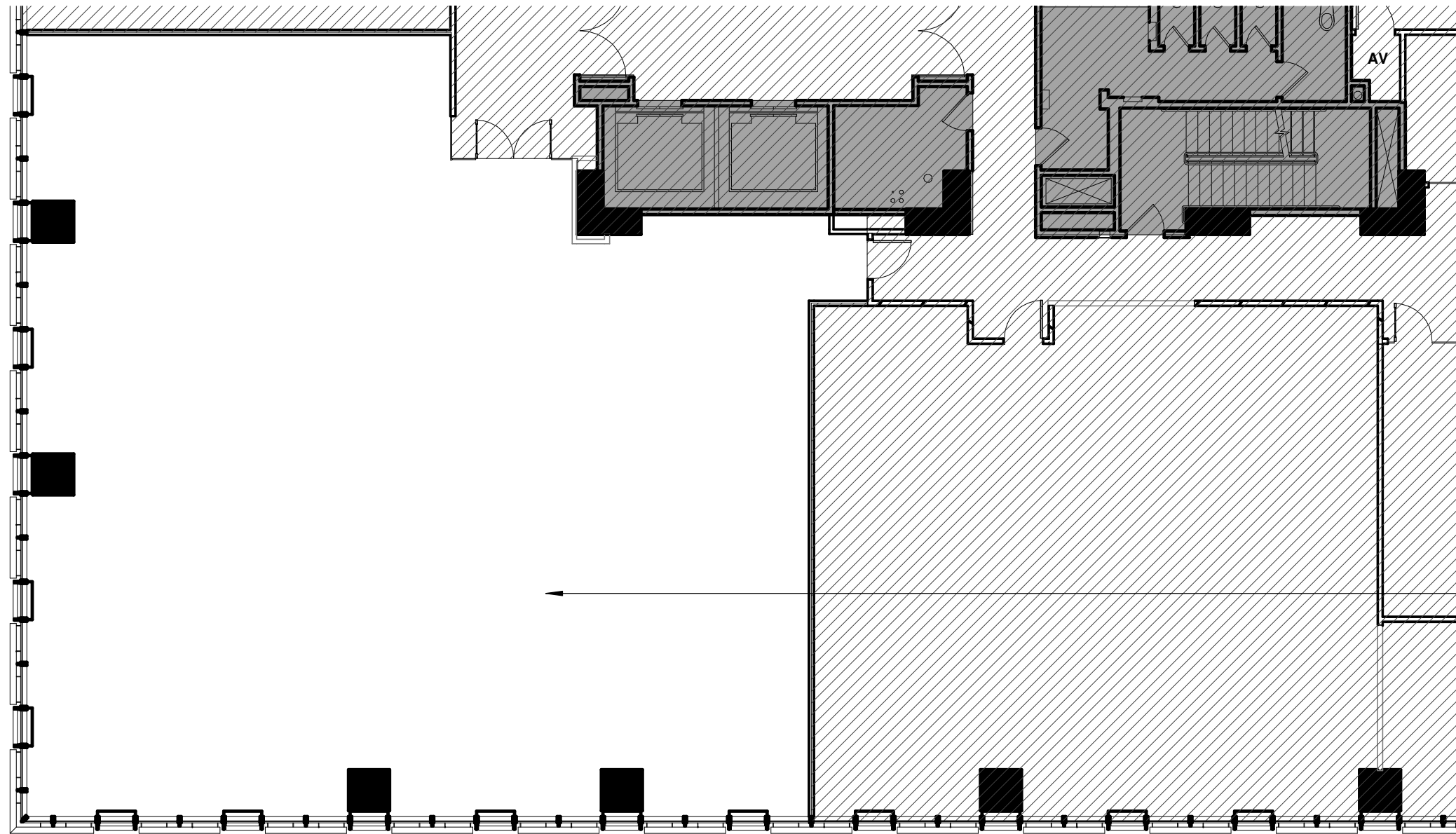
1 Level 5- Marketing Suite F 3/32" = 1'-0"
