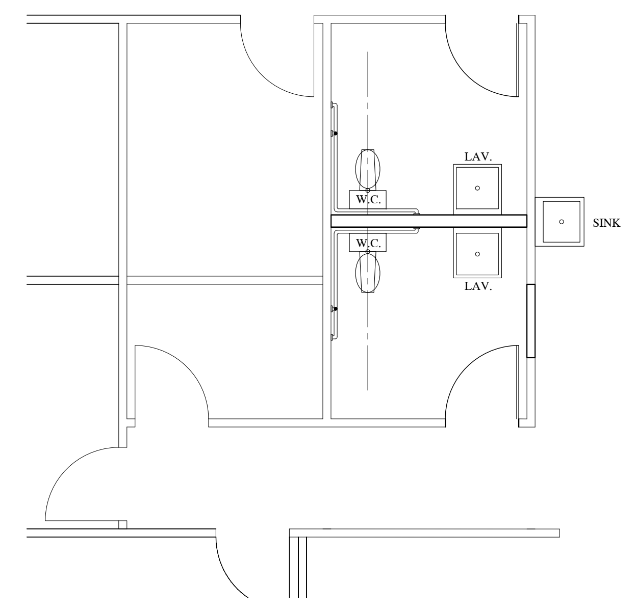
PARTIAL R/R/ PLUMBING PLAN SCALE: 1/4" = 1' - 0"
