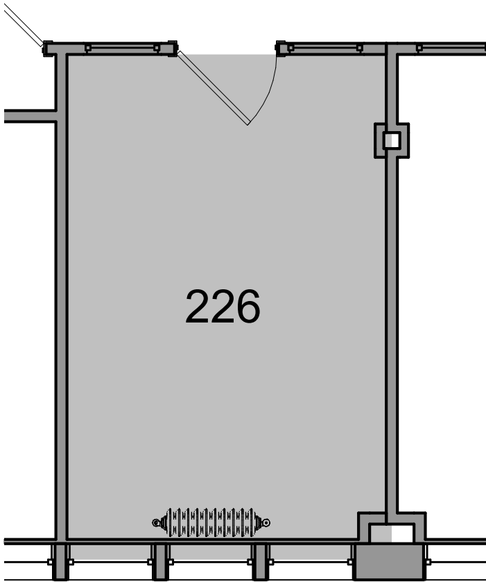
Suite 226 - Partial Existing Level 02 Plan
