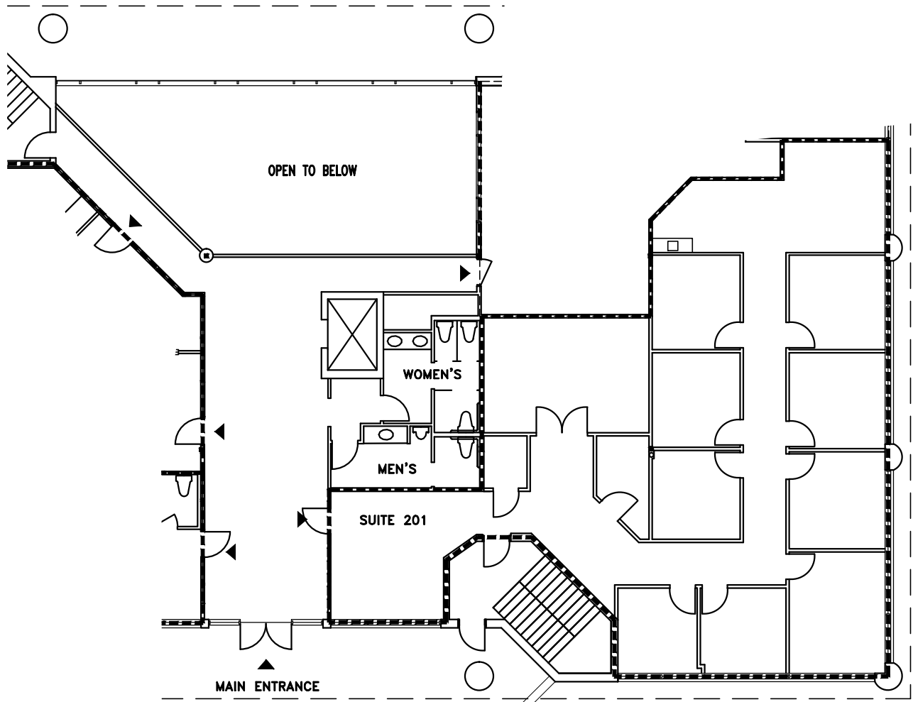
1 SECOND FLOOR PLAN—SUITE 201 SCALE 1"=16'-0"
