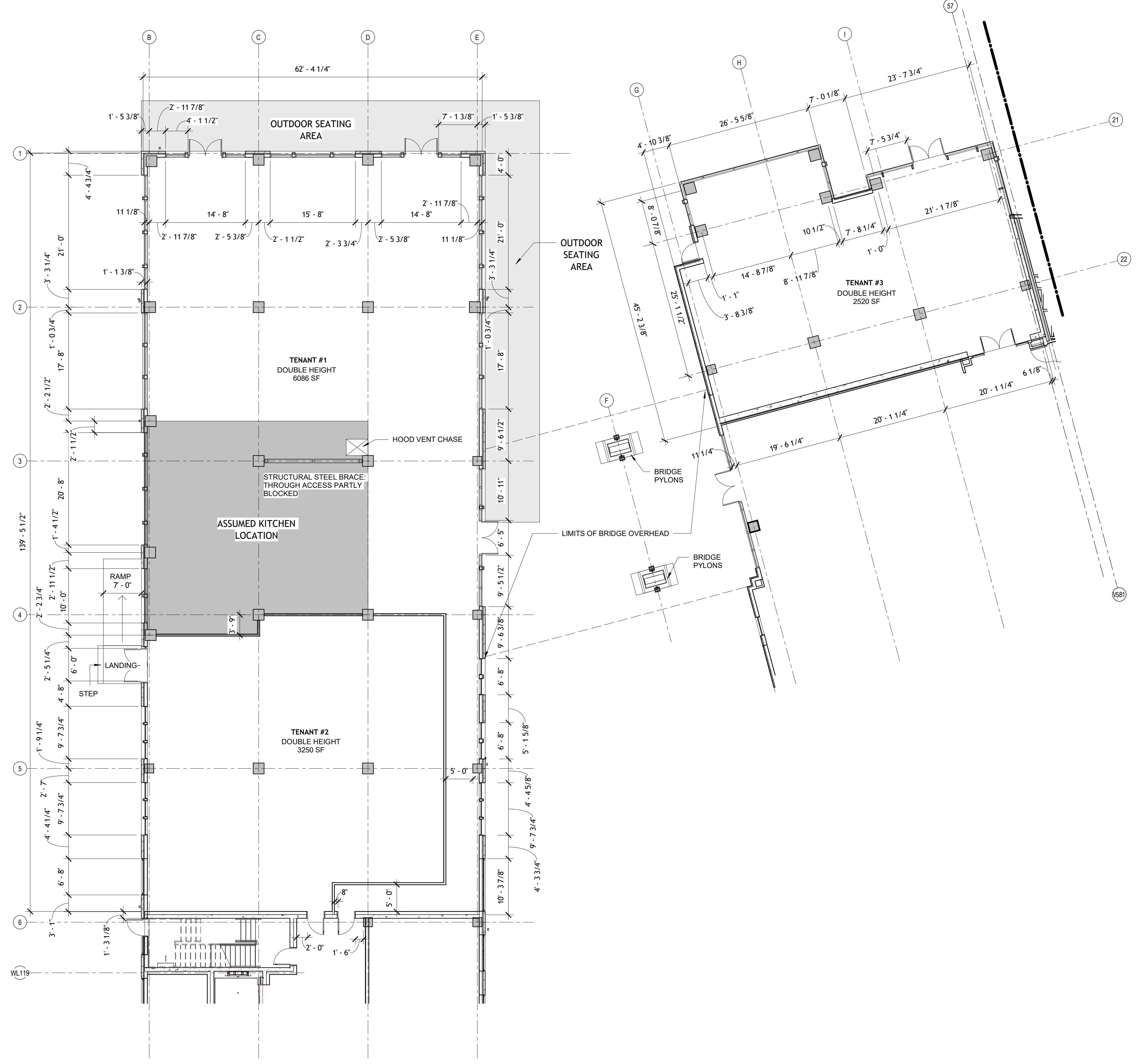
8E LOD PLAN - LEVEL 1 07 LOD 1" = 10'-0"
