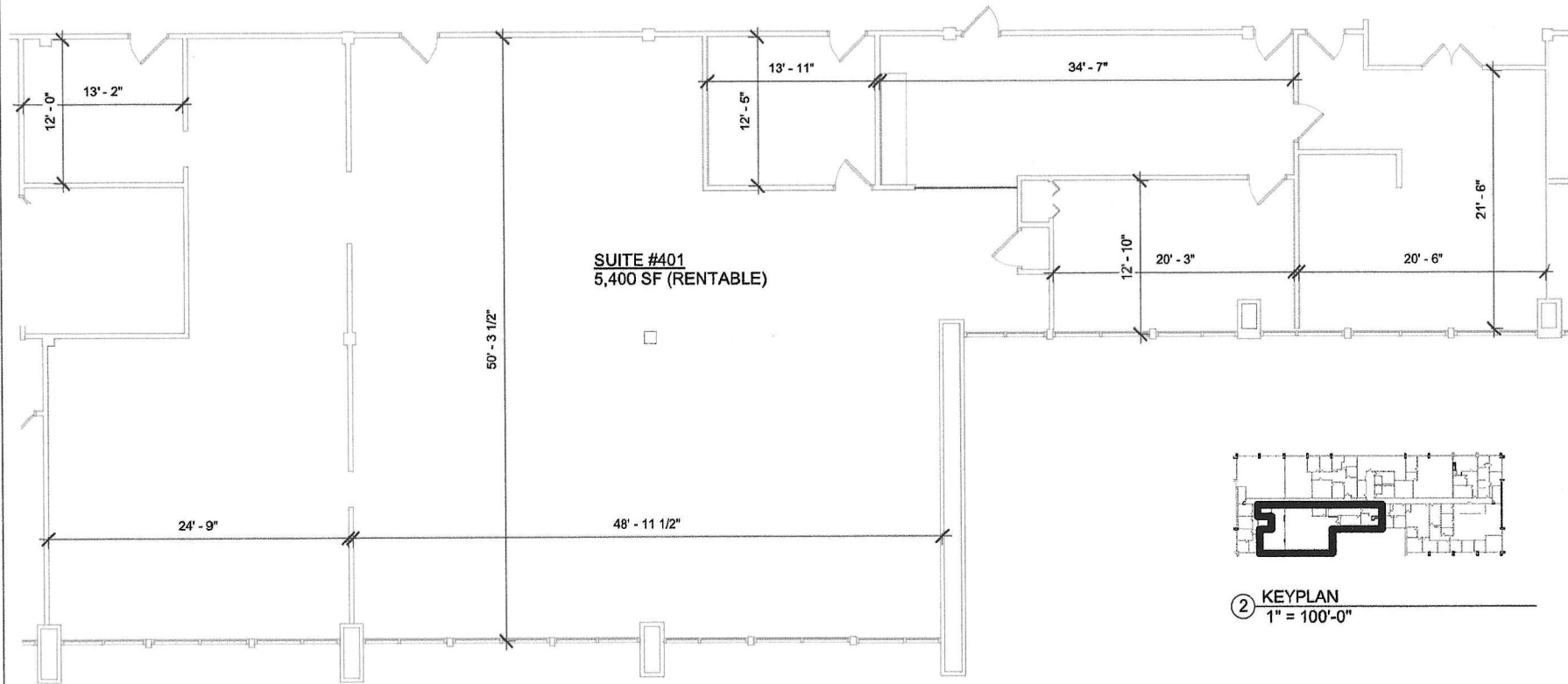
① SUITE #401 1/8" = 1'-0"
