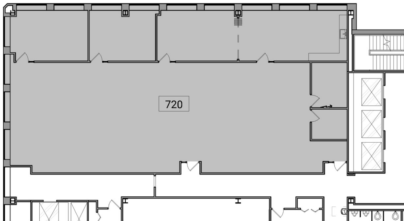
N 2 Suite 720 - Partial Level 7 Existing Floor Plan 720 8' 16' 32' 1/16" = 1'-0"
