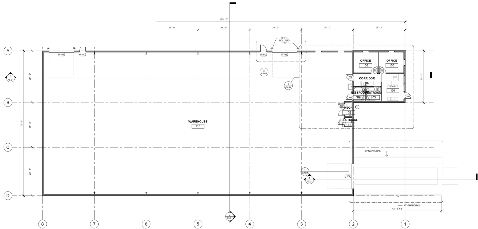
1 PROPOSED FLOOR PLAN 1/8" = 1'-0"
