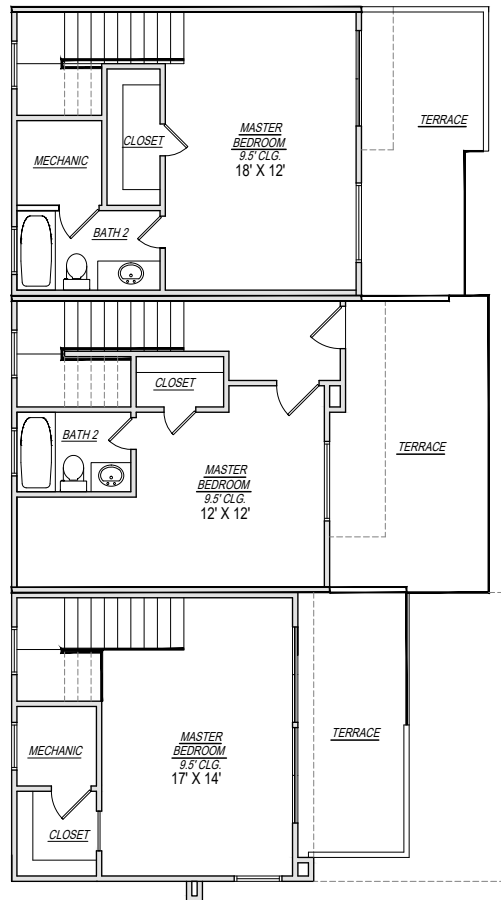
3TH FLOOR
