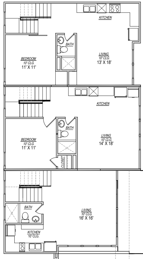
2ND FLOOR
