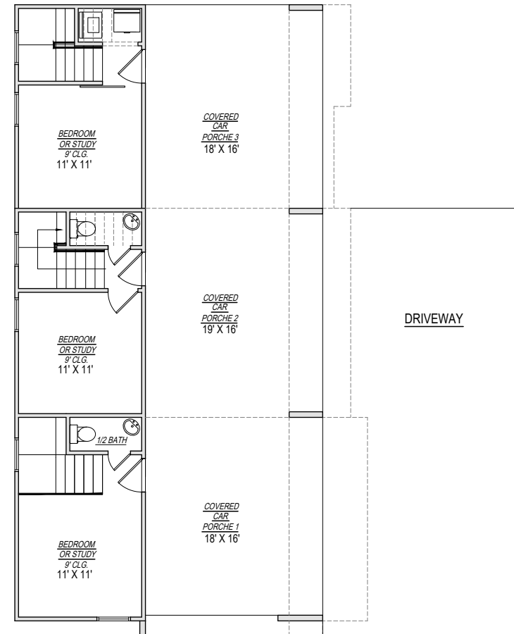
1ST FLOOR EXISTING 3 HOUSE TOTAL AREA 3800 S.F.
