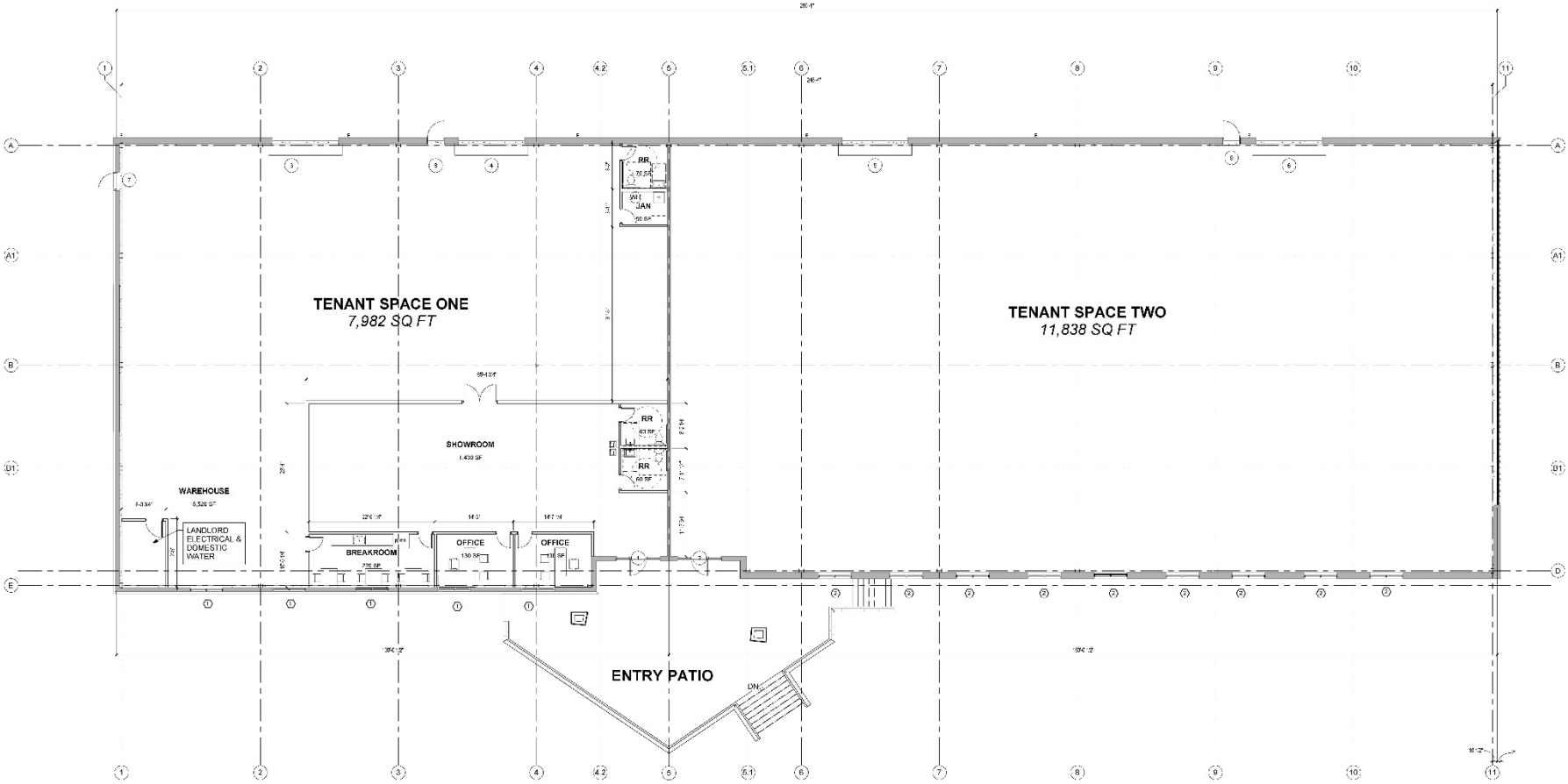
1 FIRST FLOOR PLAN 1/8" = 1'-0"
