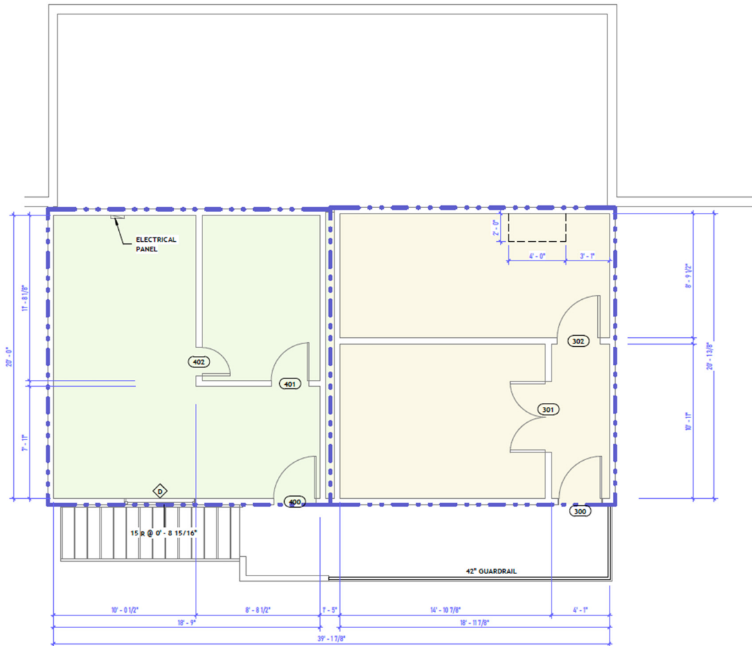
② SECOND FLOOR PLAN - OPTION 3 1/4" = 1'-0"
