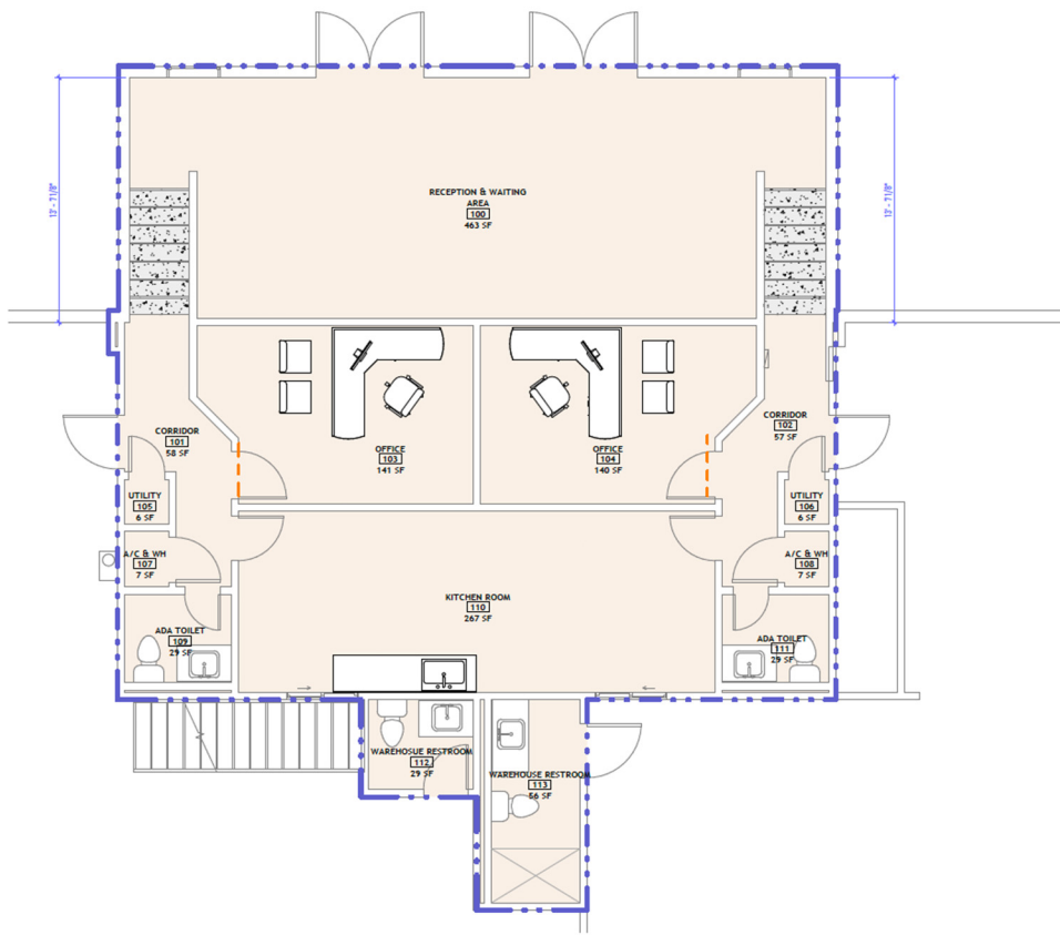
① FIRST FLOOR PLAN - OPTION 3 1/4" = 1'-0"
