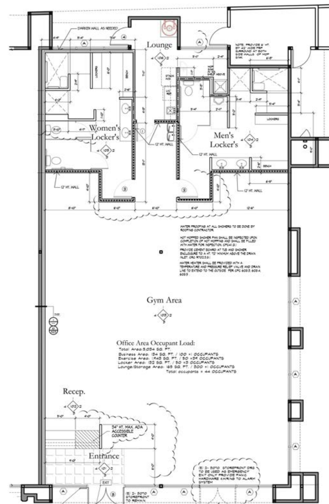
BLDG 2B: SUITES 1&2 FLOOR PLAN - 3,147 SF
