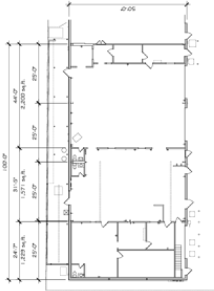
5,000 SQ.FT. EXISTING PLAN 4-11-22 5540 DIETRICH RD. suite #A SAN ANTONIO, TX. 78219
