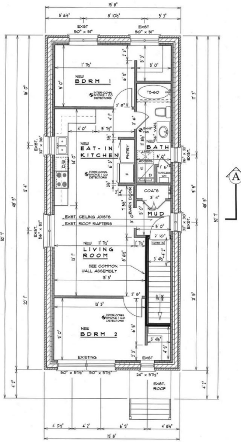
UNIT 3 2ND FLOOR PLAN
