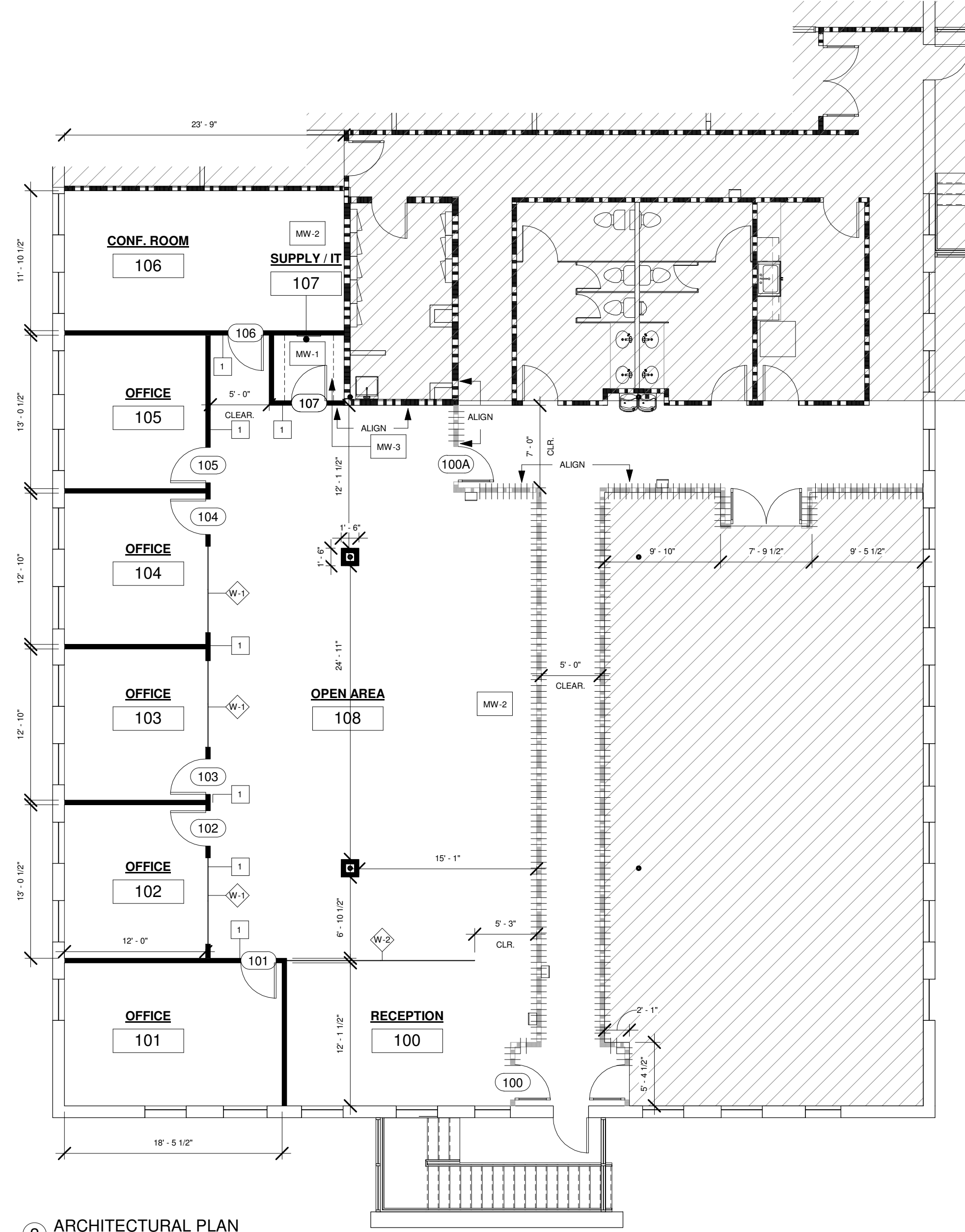
2 ARCHITECTURAL PLAN 1/8" = 1'-0"
