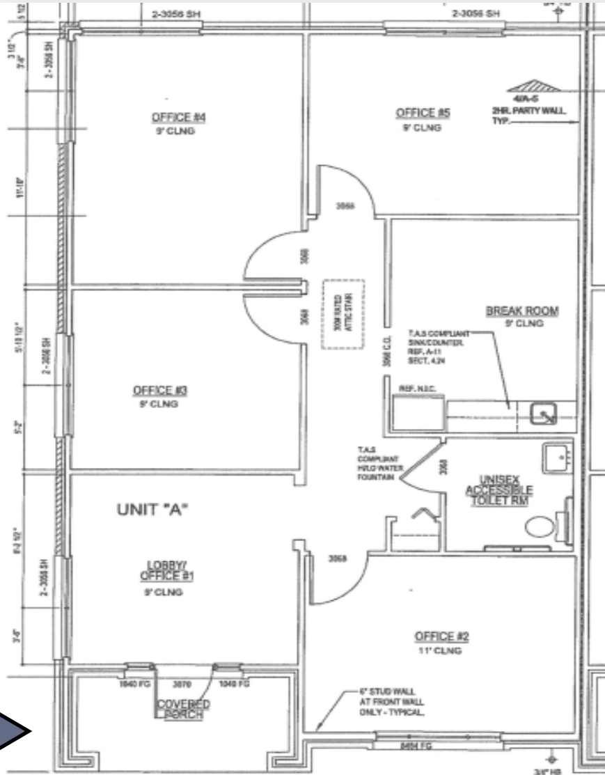
01 Floor Plan 1/4"=1'-0" 0 1 2 3 4 5 10
