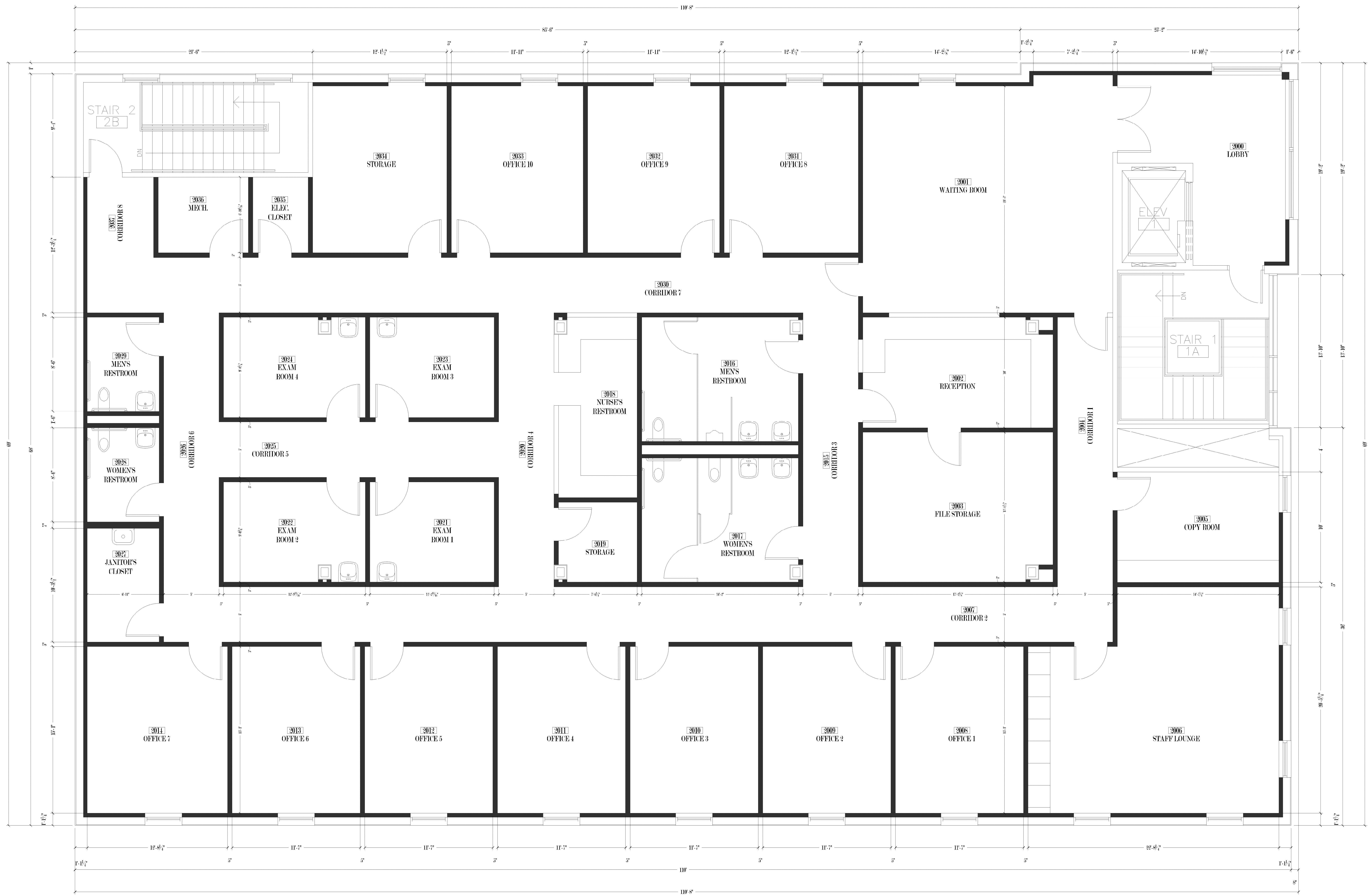
1 ROSELAND MEDICAL CENTER - SECOND FLOOR BUILDOUT PRELIMINARY OFFICE LAYOUT SCALE: 1/4" = 1'-0"
