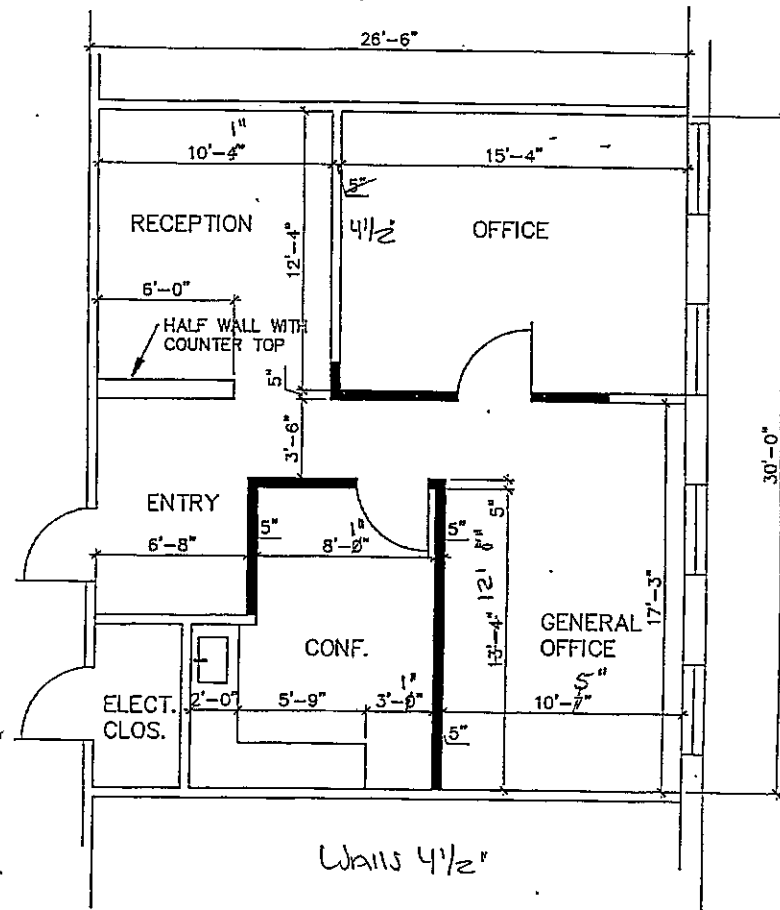
7207 FLOOR PLAN
