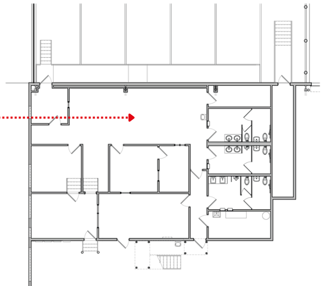
Office Plan
