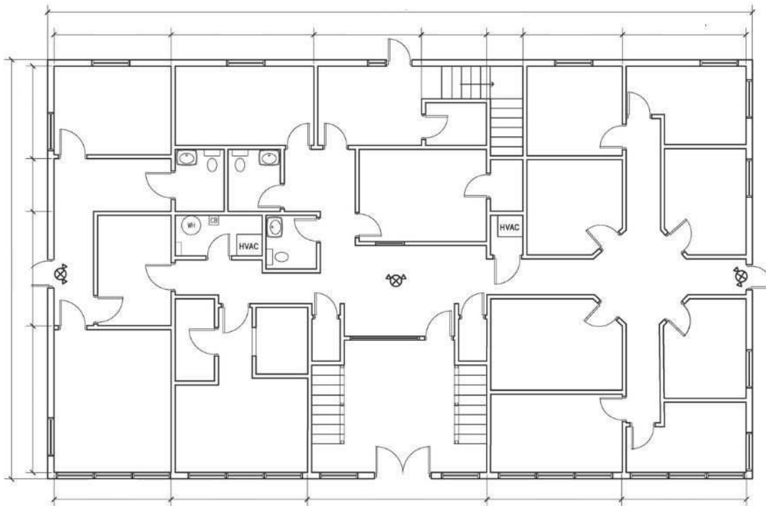
1 FLOOR PLAN 3/16" = 1'-0"
