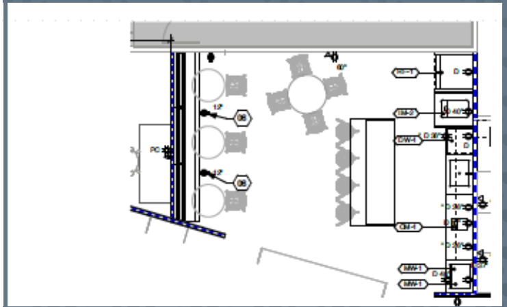
Enlarged Breakroom Power/Data Plan
