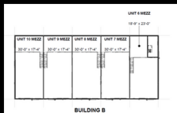
MEZZANINE LAYOUT
