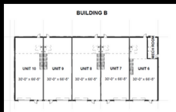
UNIT LAYOUT
