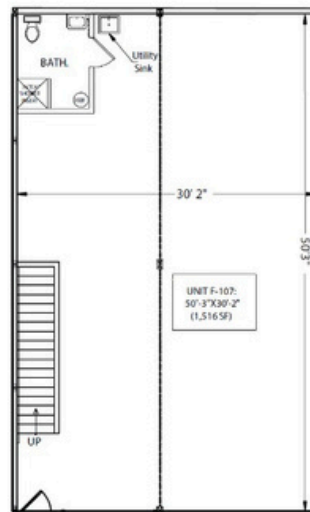
STANDARD UNIT FLOOR PLAN
