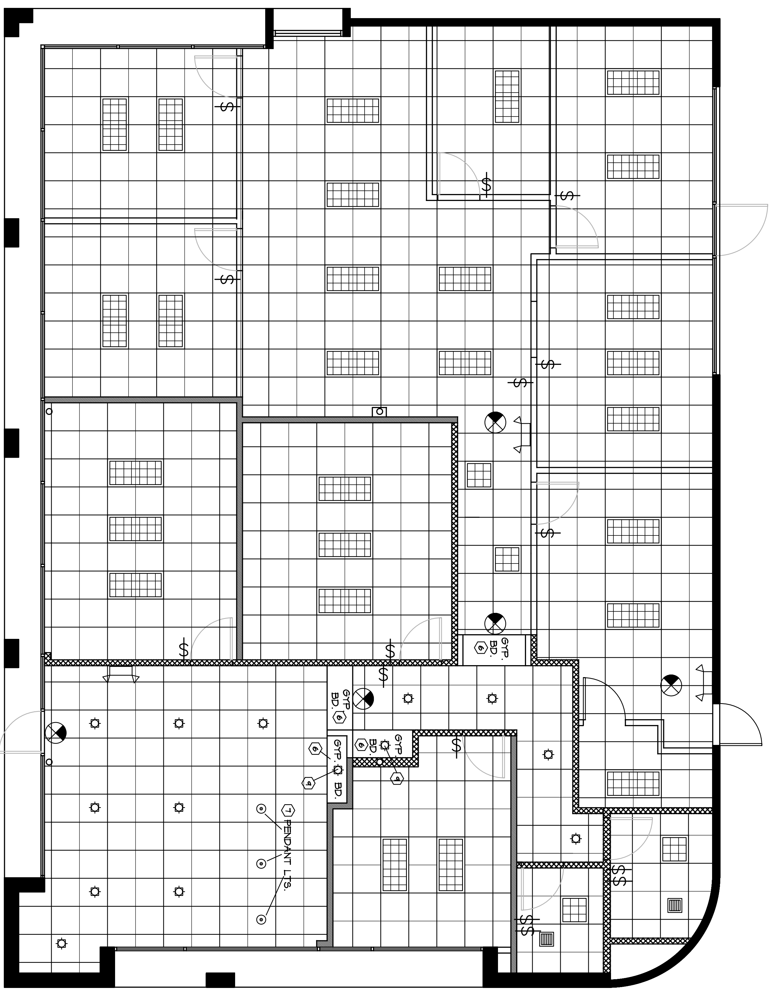
1 REFLECTED CEILING PLAN SCALE 1/4" = 1'-0"
