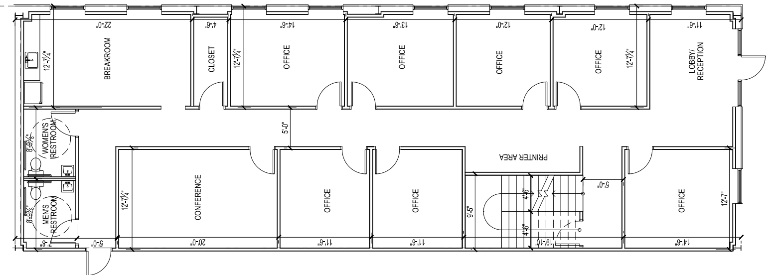
OPTION B WITH STAIRS LEADING TO SECOND STORY
