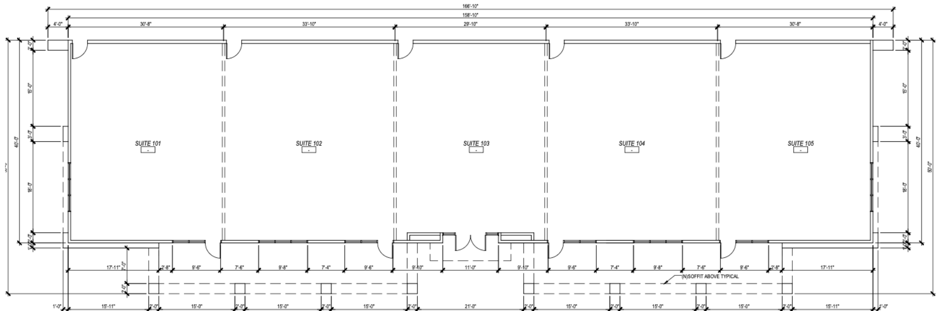
BUILDING "C" FLOOR PLAN
