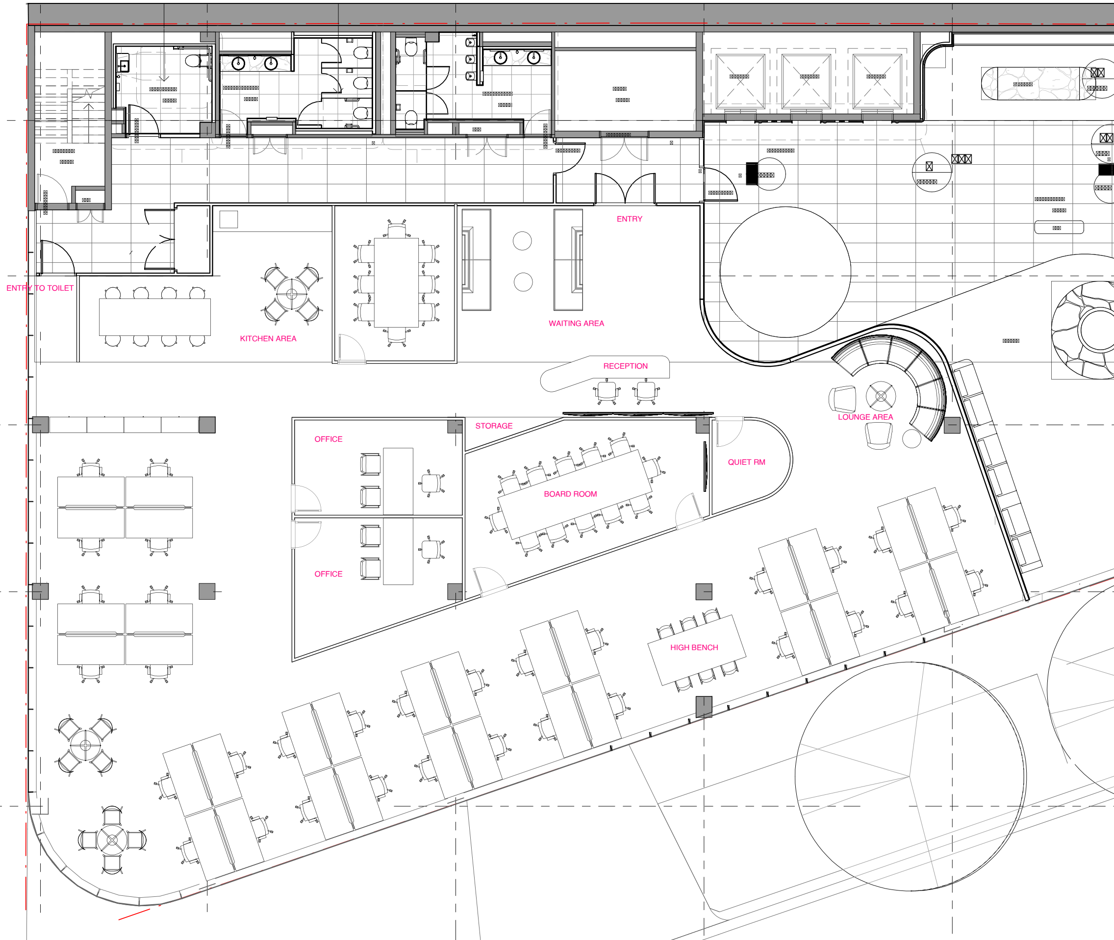
1 Proposed Floor Plan 1 : 100
