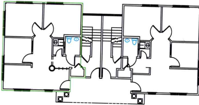
First floor - 1,830sf
