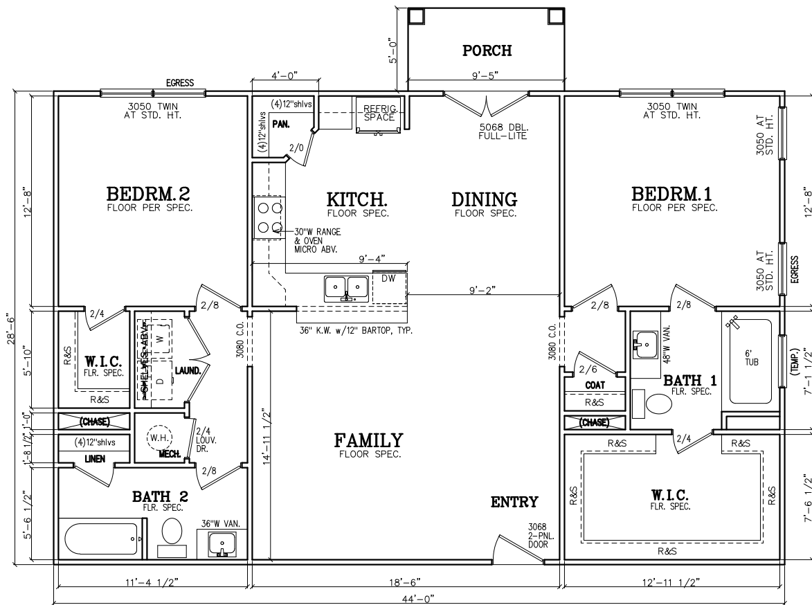
PLAN #3 FLOOR PLAN 2 BR / 2 BTH (44'-0"W x 28'-6"D)
