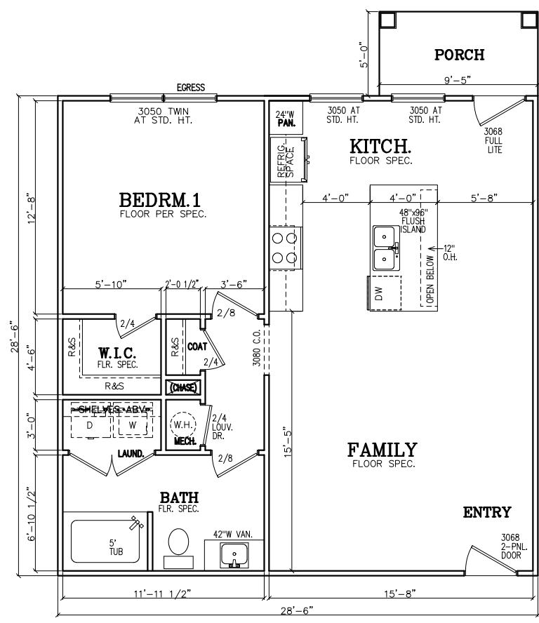
PLAN #1 FLOOR PLAN 1 BR/1 BTH - SMALL (28'-6"W x 28'-6"D)
