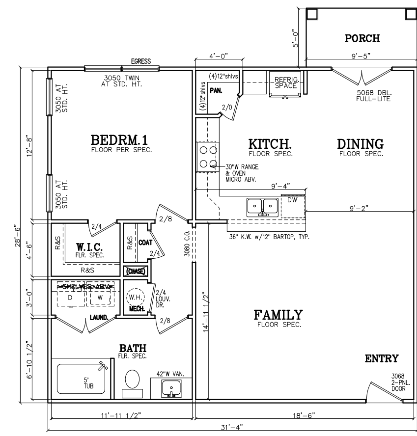
PLAN #2 FLOOR PLAN 1 BR/1 BTH - SMALL (31'-4"W x 28'-6"D)
