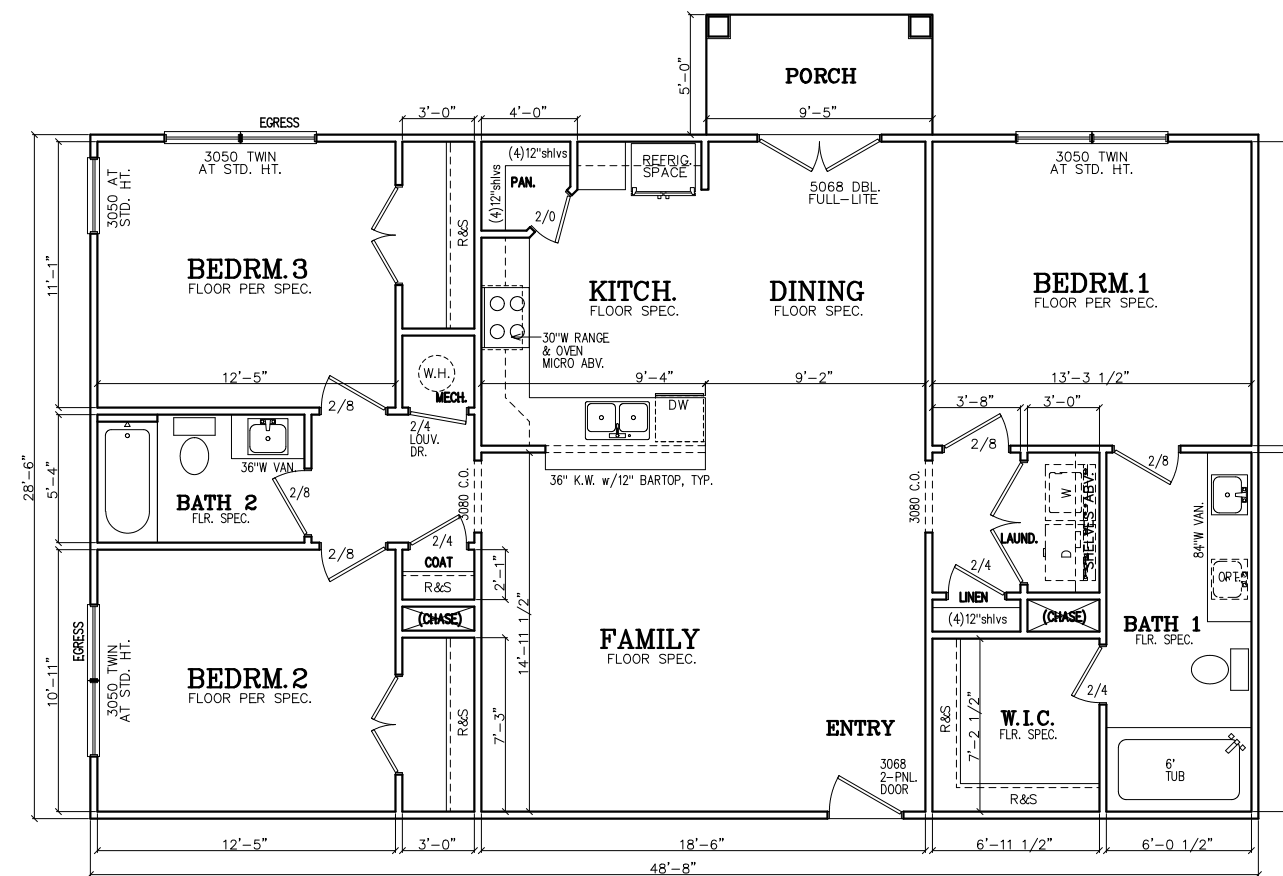
PLAN #4 FLOOR PLAN 3 BR / 2 BTH (48'-8"W x 28'-6"D)
