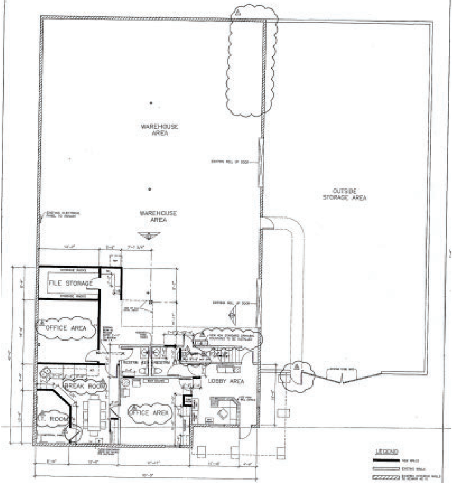
FIRST LEVEL FLOOR PLAN - PROPOSED
