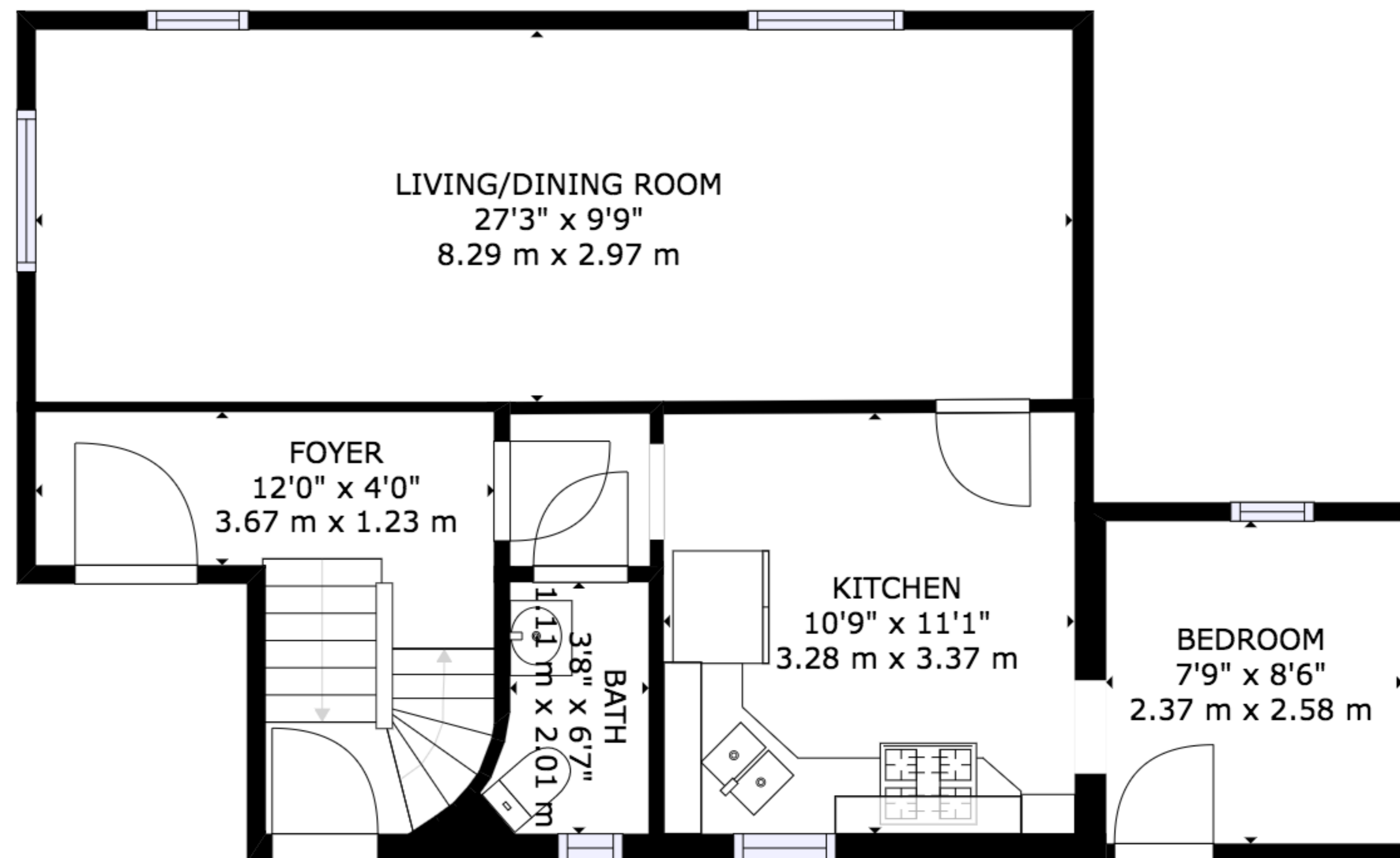
FLOOR 2
