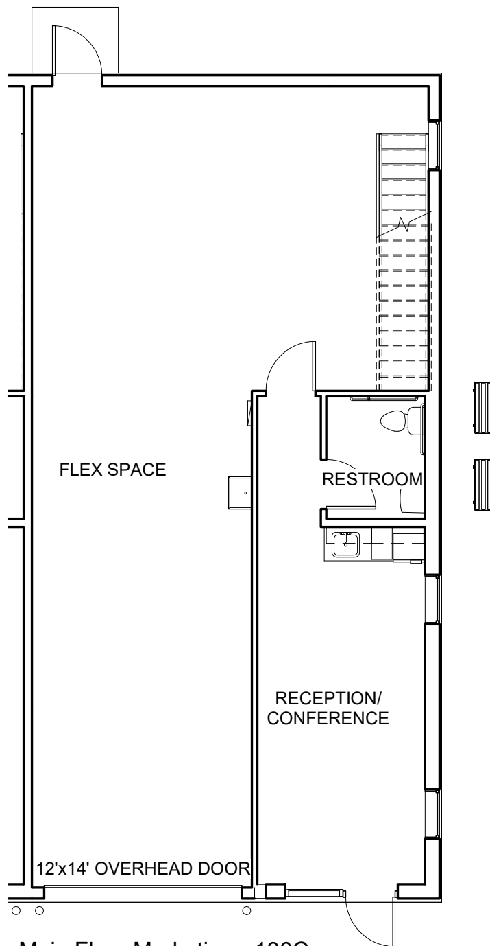
① Main Floor Marketing - 130C 1/8" = 1'-0"
